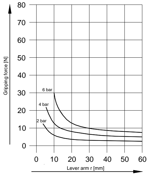
External gripping (close)
