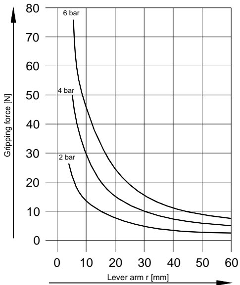
Internal gripping (open)
