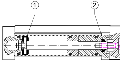
Pneumatic cylinder type B und C (size \varnothing 16 - \varnothing 40 ) 1 piston assembly 2 scraper rings
