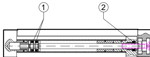
Pneumatic cylinder Typ A (size \varnothing 10 - \varnothing 40 ) Pneumatic cylinder Typ B (only size \varnothing 8 - \varnothing 10 ) Pneumatic cylinder Typ C (only size \varnothing 10 ) 1 piston seals 2 scraper ring
